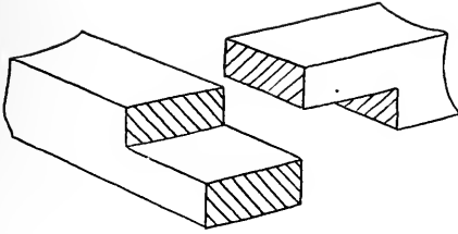
END LAP JOINT
